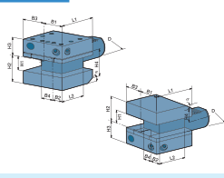
E52 Combined Static Holders
