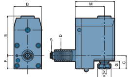
E35 Radial Drilling And Milling Heads-Backward Type
