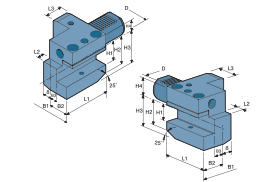
E50 Axial Static Holders
