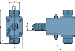
E47 Radial Drilling And Milling Heads
