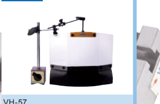
A76 Eye Shield With Magnetic Base
