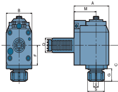
E46 Radial Drilling And Milling Heads
