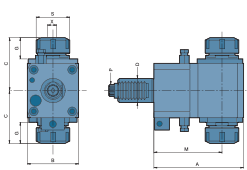
E37 Radial Double Drilling And Milling Heads
