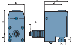
E35 Radial Drilling And Milling Heads-Backward Type
