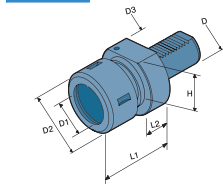
E54 Static Holders
