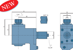
E58 H Type Milling & Drilling Head
