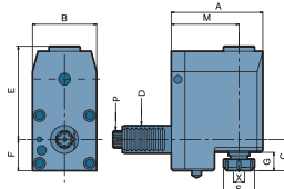
E39 Radial Drilling And Milling Heads
