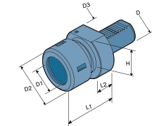
E54 Static Holders
