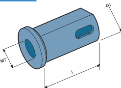
E57 Reducing Sleeves
