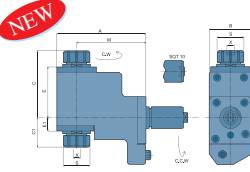
E59 H Type Milling & Drilling Head
