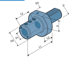
E53 Static Holders
