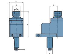
E40 Axial Drilling And Milling Heads
