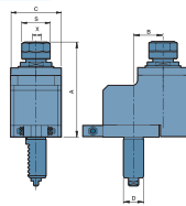
E33 Axial Drilling And Milling Heads
