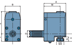
E42 Radial Drilling And Milling Heads-Backwards
