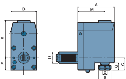
E32 Radial Drilling And Milling Heads-Back Ward Type
